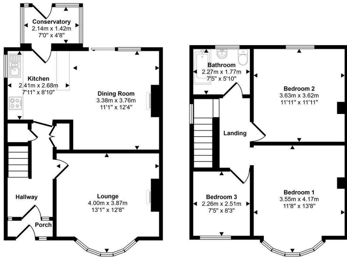
Ground Floor Approx 47 sq m / 509 sq ft
